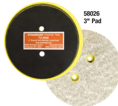
57902 Wet Dynafine®
